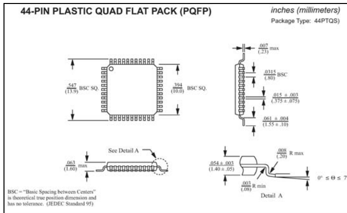
Figure 1) Current Lead Tolerances and Shape
