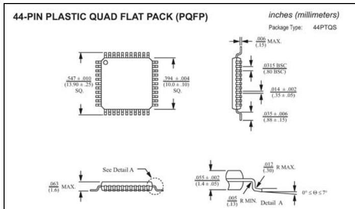
Figure 2) Retooled Lead Tolerances and Shape
