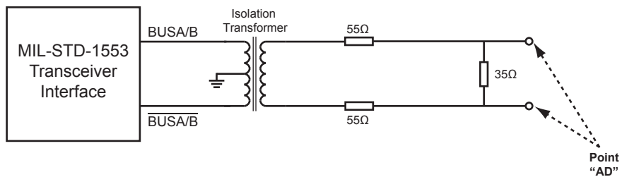
Figure 27. MIL-STD-1553 Direct Coupled Test Circuits
