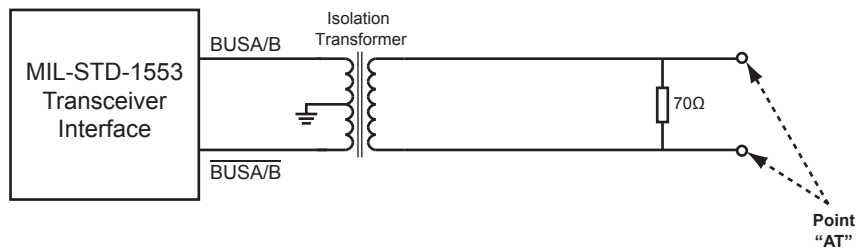
Figure 28. MIL-STD-1553 Transformer Coupled Test Circuits
