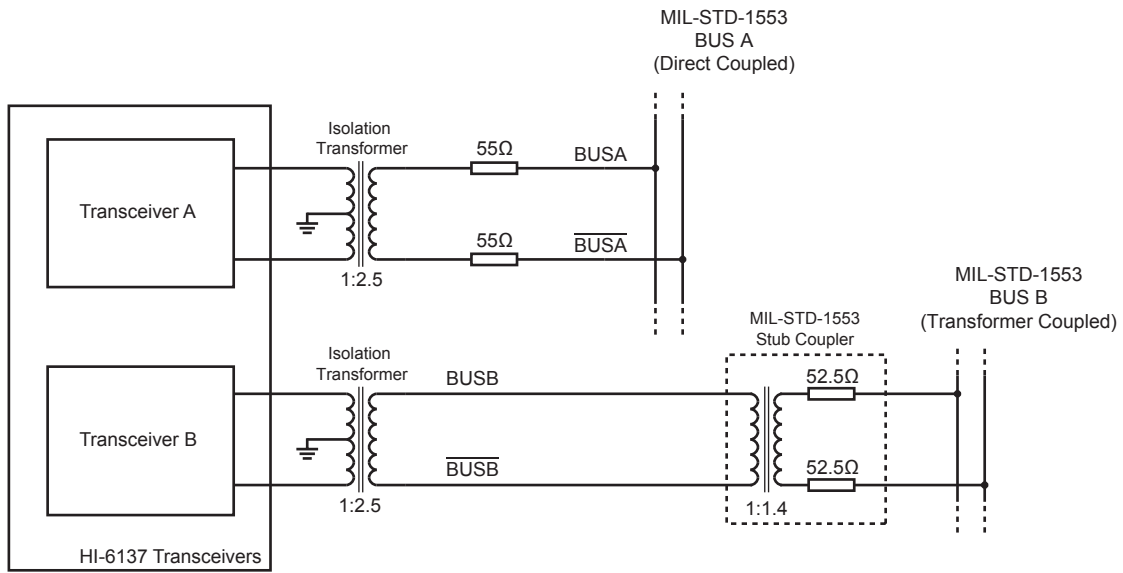
Figure 26. Bus Connection Example using HI-6137
